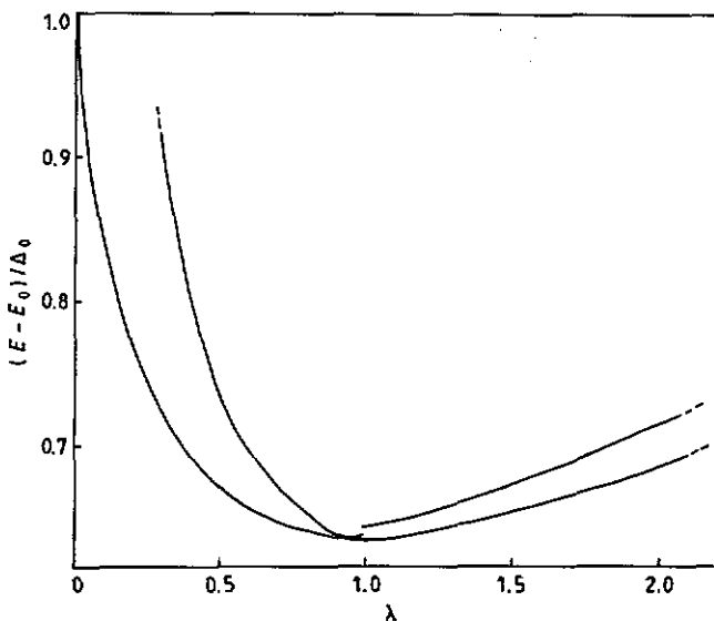
Figure 1. The exact soliton creation energy (lower curve) and the approximate soliton creation energy (upper curve) are plotted for a range of values of the 'size' parameter \lambda . The approximation for the creation energy was obtained when four MS coefficients were included in the calculation. The discontinuity appearing in the curve for the approximation at \lambda = 1 results from a new bound state being trapped on the soliton. A smoothing out of the density of bound states would avoid this feature [8].
